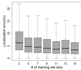
Fig. 10: Lower bound of the training set size for REAL
