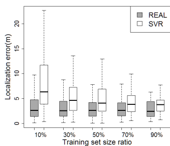
Fig. 9: Comparison of REAL vs. SVR using different size of training set
