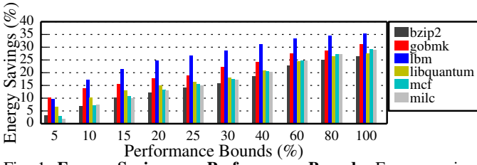
Fig. 1: Energy Savings vs. Performance Bounds: Energy savings vary across applications for a given performance bound.
