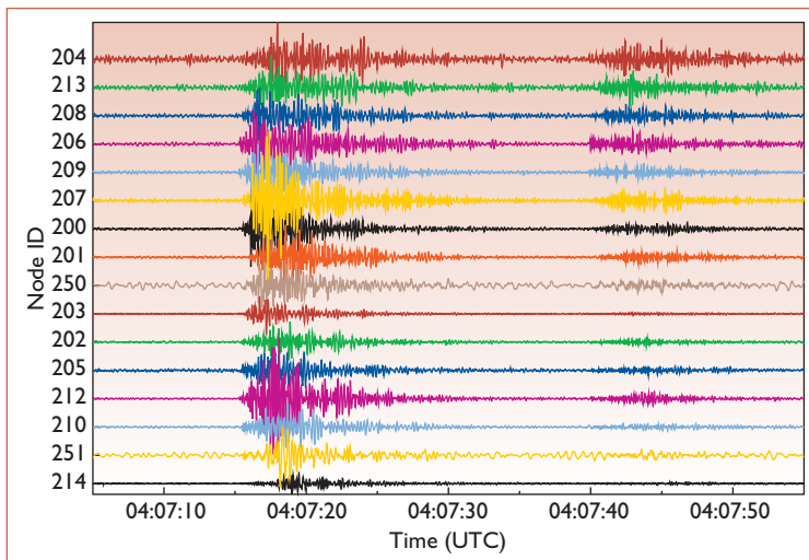
Figure 3. An event captured by our network. The event shown was a volcano tectonic (VT) event and had no interesting acoustic component. The data shown has undergone several rounds of postprocessing, including timing rectification. We show only seismic signals.
