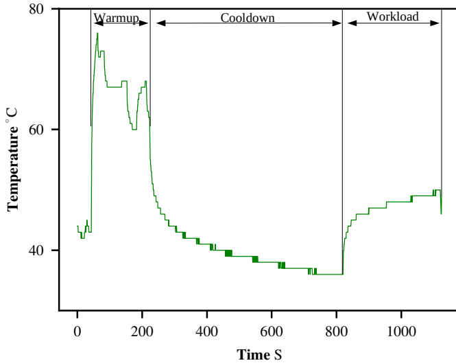
Fig. 5: Thermal characteristics during FIXED-FREQUENCY workload on Nexus 5. Due to a low frequency, the device never heats up to throttling levels.
