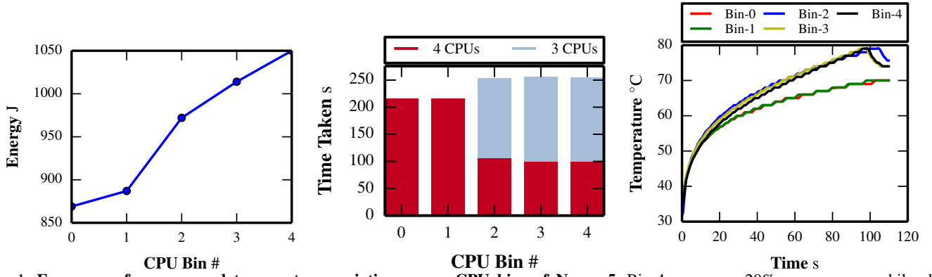
Fig. 1: Energy, performance and temperature variation across CPU bins of Nexus 5. Bin-4 consumes 20% more energy while also taking 18% longer due to thermal throttling. Once thermal limits of 80°C are reached, one CPU core is shut down.
