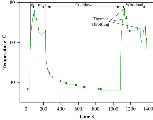
Fig. 4: Various stages of ACCUBENCH during an UNCONSTRAINED workload on Nexus 5. The warmup and cooldown phases together act as a mechanism to normalize device’s thermal state.
