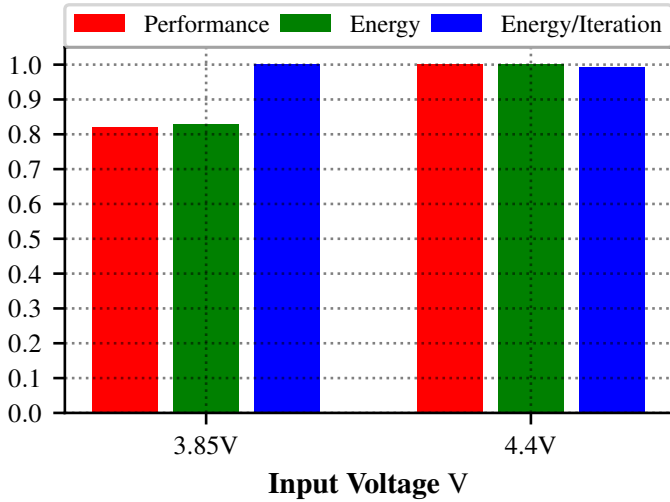
Fig. 10: LG G5 anomalous behavior . The LG G5 behaves throttled when the input voltage is set to the nominal battery voltage of 3.85V.
