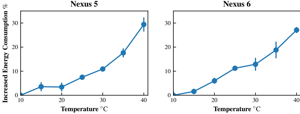
Fig. 2: Energy scaling on two different devices at max frequency. Differences in ambient temperature can cause an increase of 25% or more energy consumption to do the same work. This effect is observed across devices.
