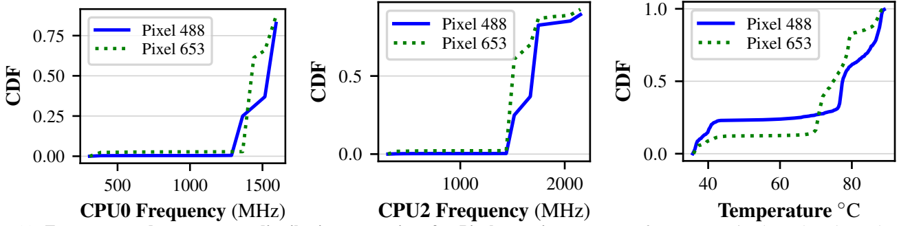
Fig. 11: Frequency and temperature distributions over time for Pixel experiments. Mean frequency varies by 7% and matches the observed performance variations.
