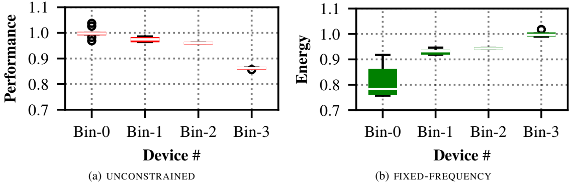
Fig. 6: Process variations in SD-800 (Nexus 5). Process variations have significant impact with observed performance and energy variations of 14% and 19% respectively.
