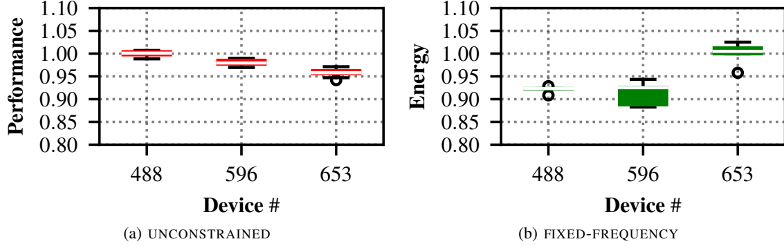
Fig. 9: Energy variations in SD-821 (Google Pixel) . Very similar behavior to the SD-820. Performance and energy variations in the order of 5% and 9% respectively.
