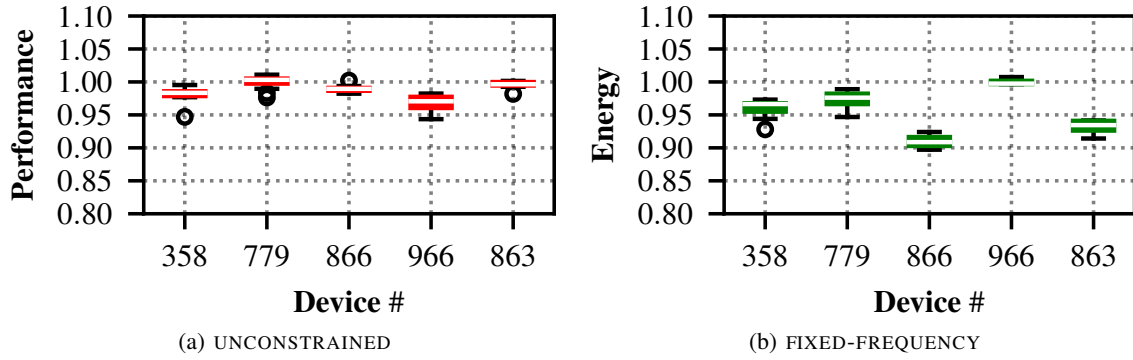
Fig. 8: Process variations in SD-820 (LG G5) . Exhibits low performance variations of 4% but energy variations of 10%.
