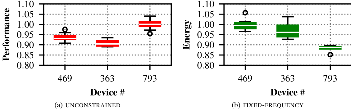
Fig. 7: Process variations in SD-810 (Nexus 6P). Performance and energy variations are in the order of 10% and 12% respectively.
