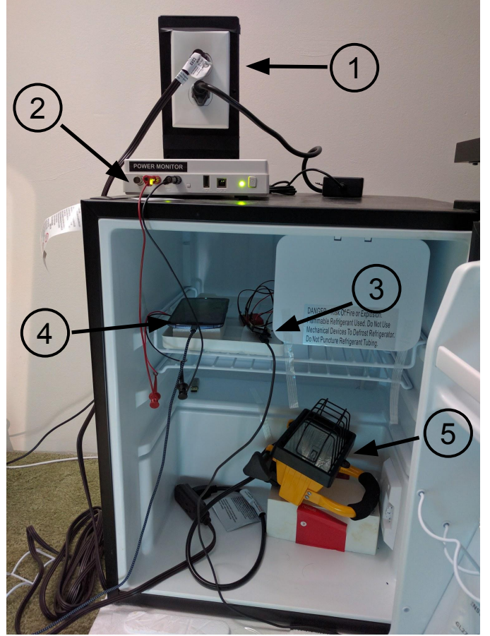
Fig. 3: Controlled thermal environment. All our experiments were run inside a controlled thermal environment with an ambient temperature of 26 \pm 0.5^\circ\text{C} . 1) Temperature Controller (RaspberryPi), 2) Monsoon, 3) ESP-8266+Thermistor (Temperature Probe), 4) Device, 5) Heating Element.
