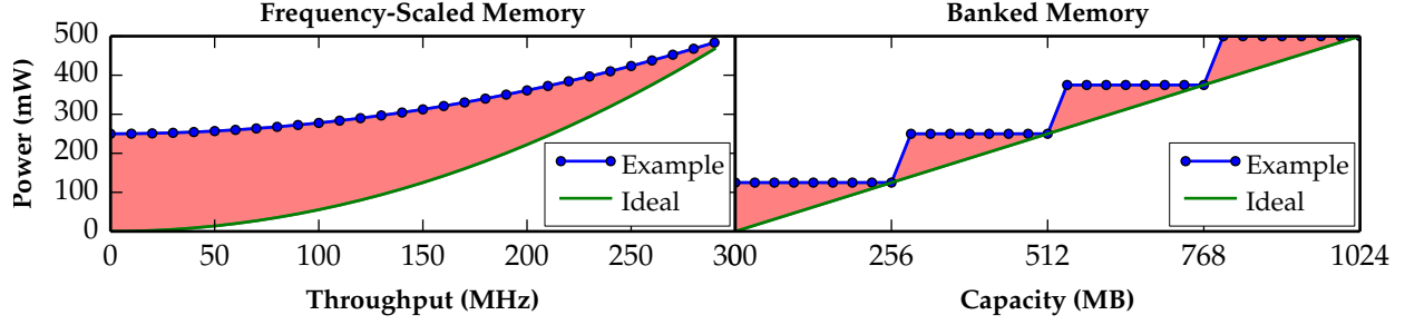
Figure 6: Example power-performance curves for two 1GB energy-proportional memory chips. Red filled areas show the degree of disproportionality with respect to an ideal component, as discussed in Section 4.2.
