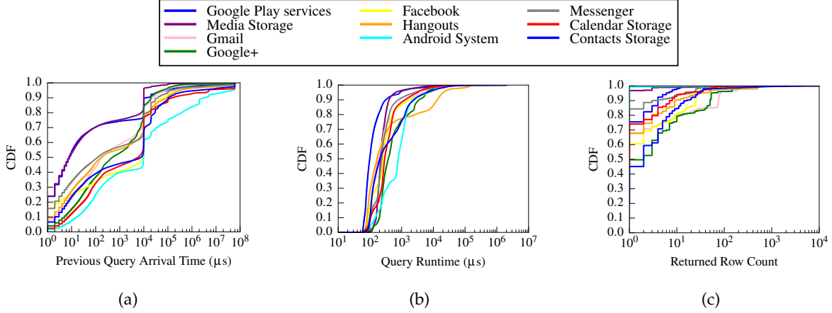
Figure 5: Per-App Summary Statistics for Android SQLite Queries. Distributions of (a) inter-query arrival times, (b) query runtimes, and (c) rows returned per query.
